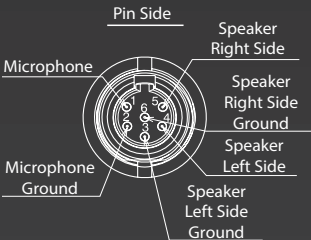
Pin Configuration for -110 Headset
